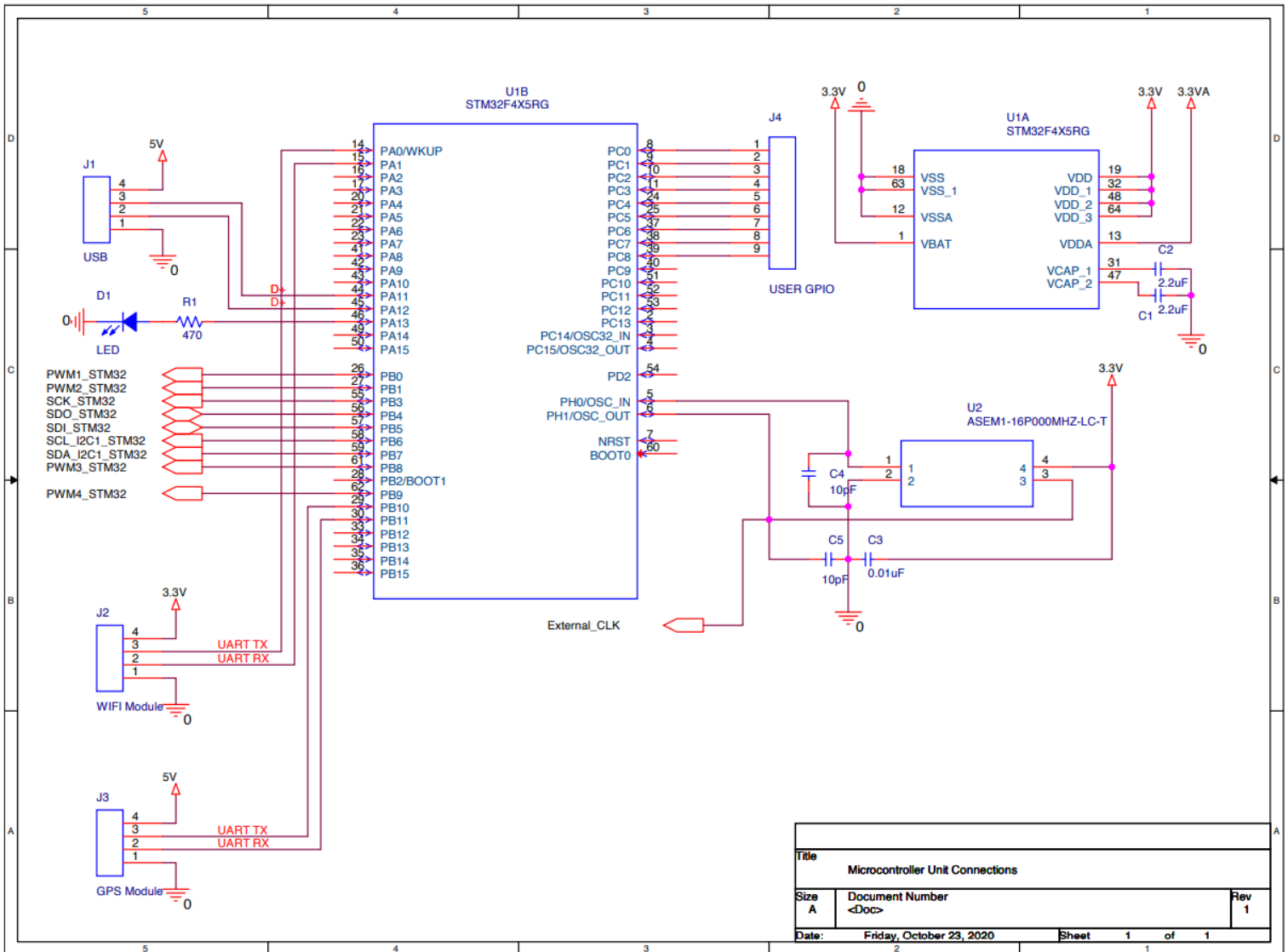
Figure 2: Microcontroller Connections Schematic
